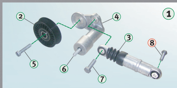
Figure 1: Detailed illustration of 55480 including all components
